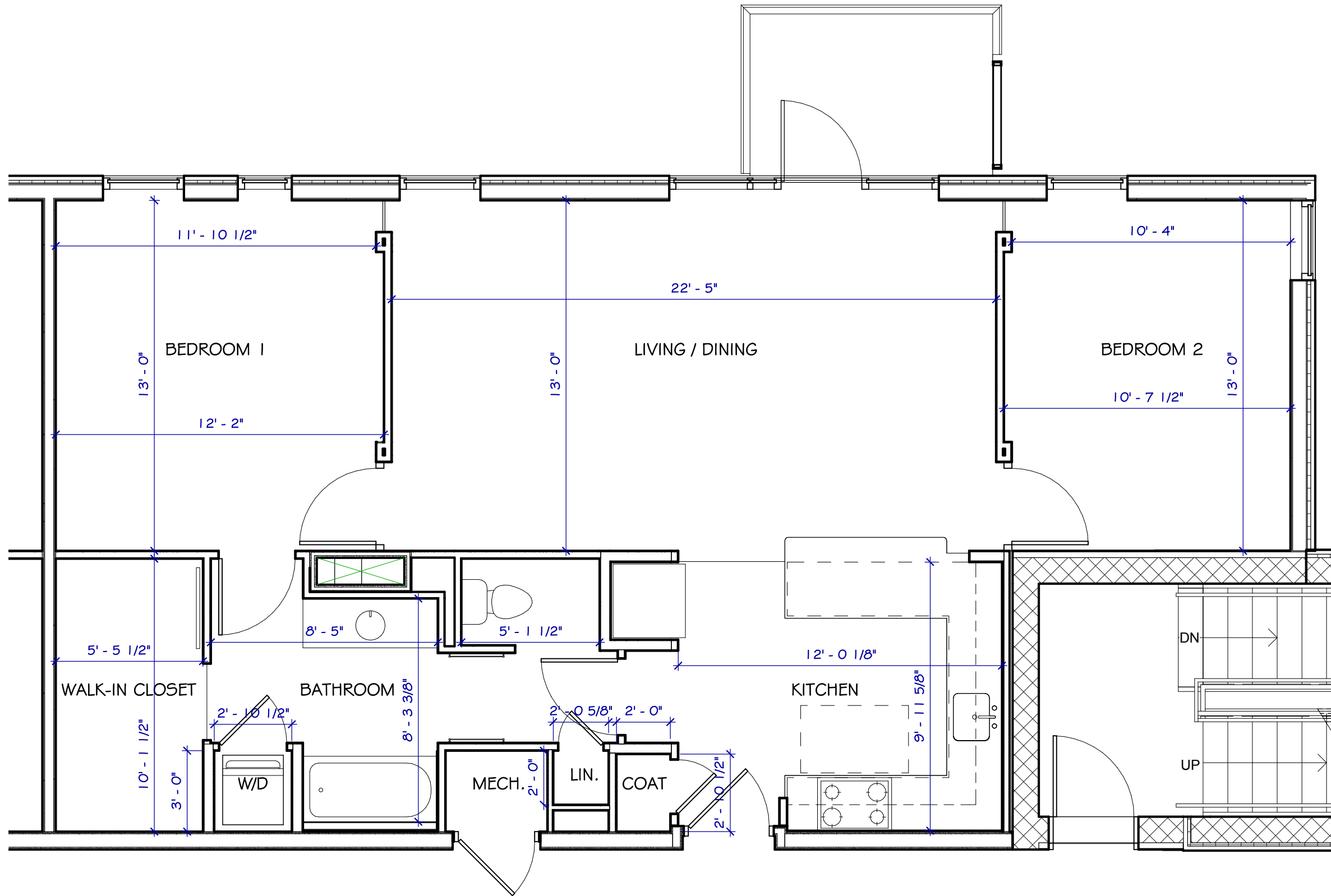
2 Unit B Plan Scale: 1/4" = 1'-0"
