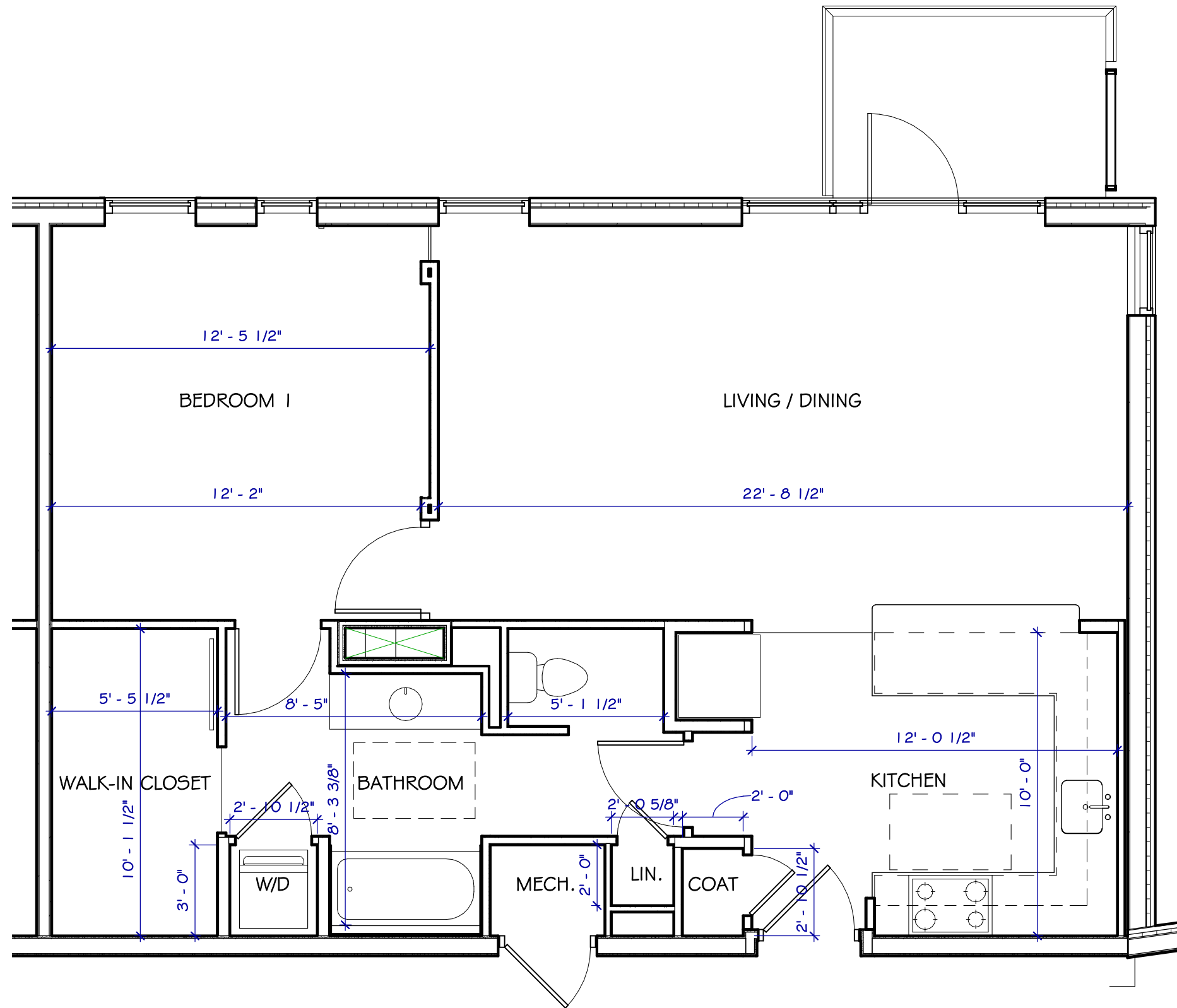
1 Unit A Plan Scale: 1/4" = 1'-0"
