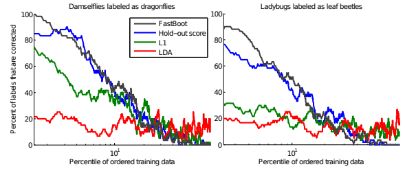
Figure 5. Percent of leaf beetle/dragonfly images that are truly ladybugs/damsselfies, when sorted by 1) median dissimilarity to the ladybug/damsselfy data set (sliding window of size 61), 2) cross-validation scores, 3) median L1 distance to the ladybug/damsselfy data set and 4) median LDA distance to ladybug/damsselfy data set.
