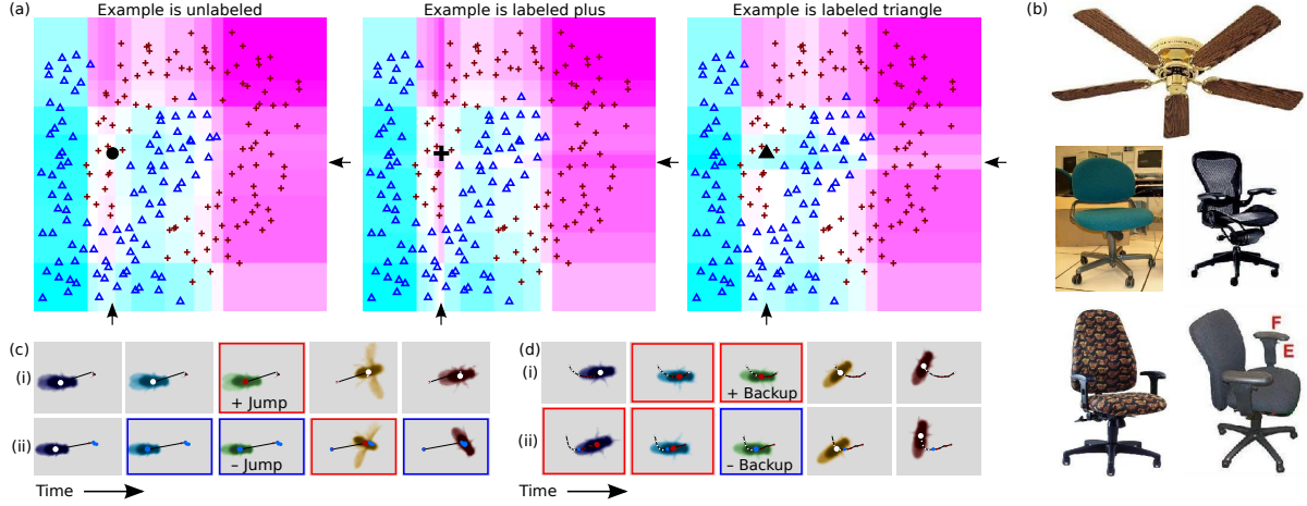
Figure 1. (a) Illustration of the influence of an example. Two classes of training data are indicated by + (red pluses) and \triangle (blue triangles). If we add the example indicated by the black circle to the training data set with the plus and triangle labels, the predictions of the classifiers learned using boosting (indicated by the color and intensity of the image) change in certain parts of the space. In particular, we see a magenta column when we add the example as red plus, and a cyan row when we add the example as a blue triangle. The effect of changing the example’s label is a function of both the learning algorithm (boosted decision stumps) and the distribution of the data. (b) Images of a ceiling fan and chairs from the Caltech 101 data set [12] that look similar to an object detector. If an object detector predicted this fan was a chair, without the context that some chairs have fan-shaped bases, it would be difficult to understand the cause of this error. (c) Example of a labeling mistake in a data set used for training a “jump” behavior classifier for flies. (d) Example of inconsistently labeled data in a training set used to train a “backup” behavior classifier for flies. The central frames are virtually identical, but were given opposite labels by the user. The training label is indicated by the box color (red = positive, blue = negative), and surrounding frames show temporal context. (c-d) were found automatically using our method to analyze the training data sets.
