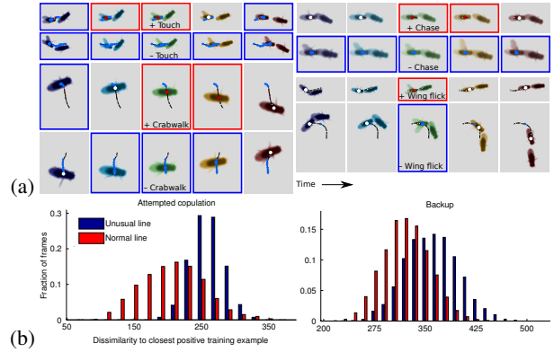
Figure 4. (a) Similar looking examples with opposite labels, plotted as Figure 1(c-d). The center frame shows the two training examples with opposite labels that are closest according to the FastBoot distance (two more are shown in Figure 1(c-d)). (b) Distribution of dissimilarity of predicted positives to the training data for two behavior data sets. We show the distribution for an ‘unusual’ fly line for which the classifier performs poorly and a ‘normal’ fly line for which the classifier performs well.
