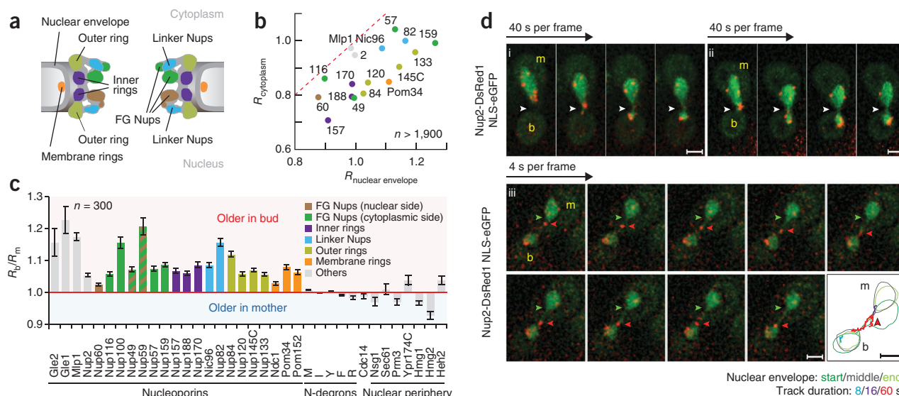
Figure 3 Inheritance of nuclear pore complexes during yeast mitosis. (a) Relative position of different structural elements of the NPC, according to reference 46. (b) Comparison of mCherry/sfGFP intensity ratios ( R ) of the indicated nucleoporins (e.g., Nup60 abbreviated as 60) at the nuclear envelope and in the cytoplasm. Colors indicate the structural assignments according to a . Intensity ratios at the red dashed line are equal in the two compartments. Error bars (s.e.m.) are smaller than the symbols representing the data points. (c) mCherry/sfGFP intensity ratios of the indicated proteins fused to mCherry-sfGFP were measured in mother ( R_m ) and bud ( R_b ) compartments at the nuclear envelope (nucleoporins, nuclear periphery proteins), in the nucleolus (Cdc14) or in the cytoplasm. Symmetrically localized nucleoporins with phenylalanine-glycine (FG) repeats (FG Nups) are colored in green/brown. Error bars indicate s.e.m. The difference between R_m and R_b is significant for all nucleoporins ( P < 0.006 in an unpaired t -test) except Gle2 ( P > 0.01 ). (d) (i, ii) Movement of Nup2-DsRed1 dots in early anaphase relative to the bud neck (white arrowheads). (iii) A single Nup2-DsRed1 dot (red arrowheads) moves from the base of the mother nucleus (green arrowheads) into the bud. Tracks of NPC movement are color coded according to duration; tracking stopped when the NPCs moved out of focus; arrowhead indicates initial direction of movement. Mother (m) and bud (b) compartments are indicated. Scale bars, 2 \mu\text{m} .
