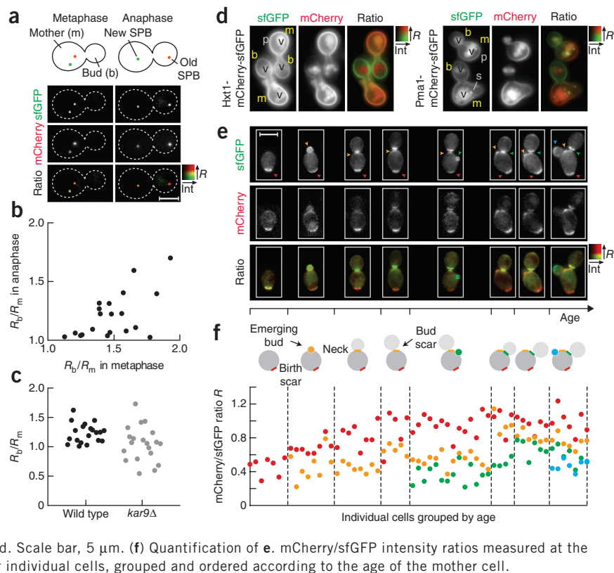
Figure 2 Analysis of differential inheritance of cellular structures with the mCherry-sfGFP timer. (a–c) mCherry/sfGFP intensity ratios of Spc42-mCherry-sfGFP at SPBs retained in the mother ( R_m ) and at SPBs directed toward or in the bud ( R_b ). (a) Ratiometric images (bottom panel) are color-coded according to sfGFP intensity (Int) and intensity ratio R , as indicated. Scale bar, 3 \mu m. (b) R_b/R_m ratios in cells from a followed with time-lapse microscopy. Each point corresponds to a single cell analyzed in metaphase ( t = 0 min) and at the end of anaphase ( t = 30 min). (c) R_b/R_m ratios in wild type and kar9 \Delta cells at the end of anaphase. (d) mCherry/sfGFP intensity ratios of Hxt1 and Pma1 fusions at the plasma membrane (p), vacuoles (v) and secretory compartments (s) in mother (m) and bud (b) cells. Ratiometric mCherry/sfGFP images are color-coded as indicated. Scale bar, 5 \mu m. (e,f) mCherry/sfGFP intensity ratios of structures marked with Rax2-mCherry-sfGFP. (e) Images of representative diploid cells ordered according to cell age and cell cycle stage. Different structures are marked with arrowheads according to origin (red, birth; orange, first cell cycle; green, second cell cycle; cyan, third cell cycle). Ratiometric mCherry/sfGFP images are color-coded as indicated. Scale bar, 5 \mu m. (f) Quantification of e . mCherry/sfGFP intensity ratios measured at the structures indicated in the cartoons are plotted for individual cells, grouped and ordered according to the age of the mother cell.
