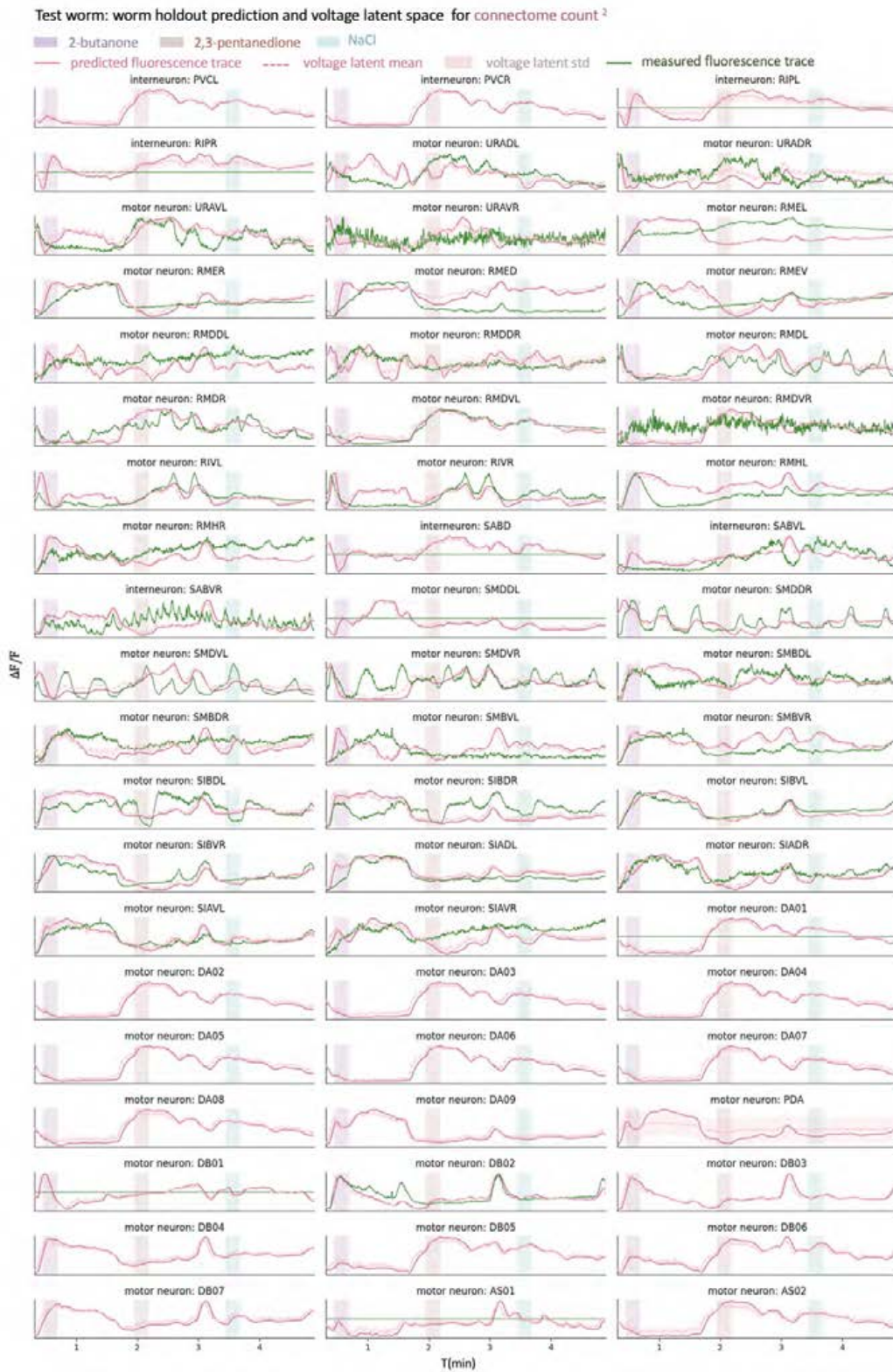
Figure 19: A hold-out (test) worm evaluated on worm holdout using connectome count 2 constraint : CC-LVM predicted traces and the corresponding voltage latent space across all neurons including unmeasured neurons (part 4).
