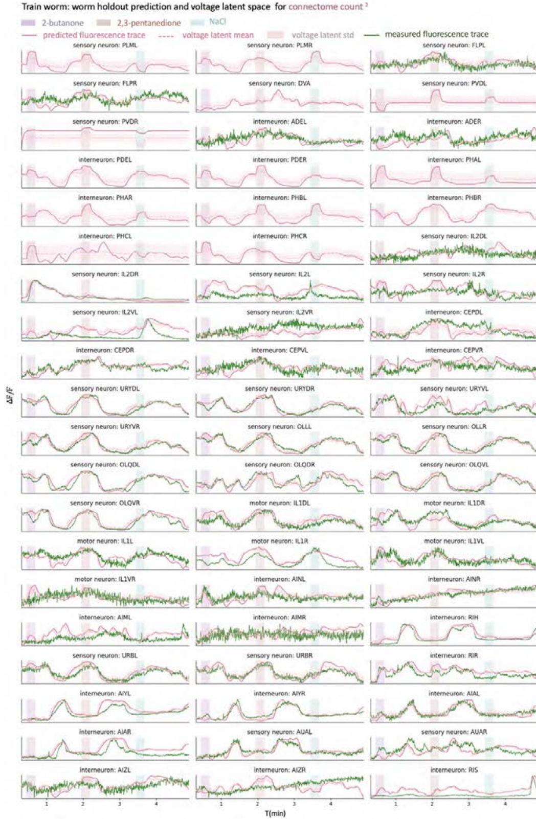
Figure 12: A train worm evaluated on worm holdout using connectome count 2 constraint: CC-LVM predicted traces and the corresponding voltage latent space across all neurons including unmeasured neurons (part 2).
