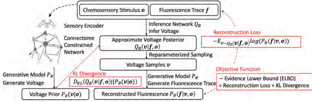
Figure 3: Schematic of the connectome-constrained latent variable model (CC-LVM). Sensory inputs are fed through a biophysically realistic connectome-constrained network to generate the voltage prior P_\theta(v|o) . To train the model, we first used an inference network to infer from the data the approximate voltage posterior Q_\phi(v|f) . Fluorescence traces are then reconstructed via a generative model P_\theta(f|v, o) . We then compared the reconstructed fluorescence traces to the measured traces, and optimized the model with evidence lower bound (ELBO), with a combination of reconstruction loss and KL divergence.
