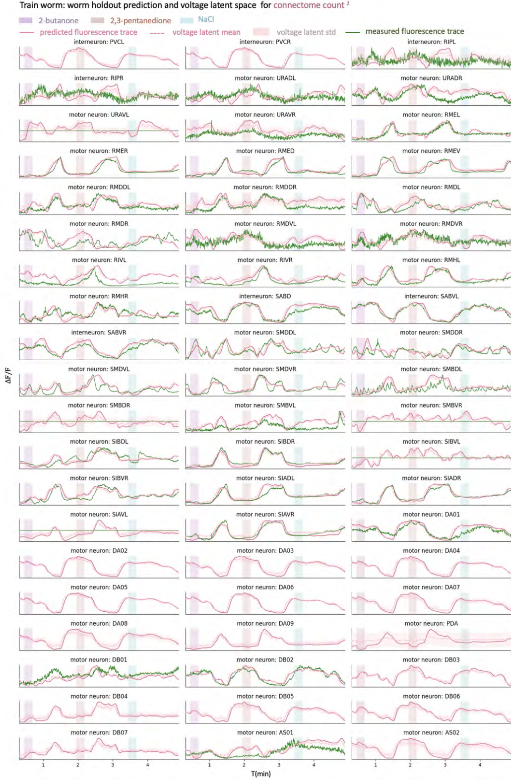
Figure 14: A train worm evaluated on worm holdout using connectome count 2 constraint: CC-LVM predicted traces and the corresponding voltage latent space across all neurons including unmeasured neurons (part 4).
