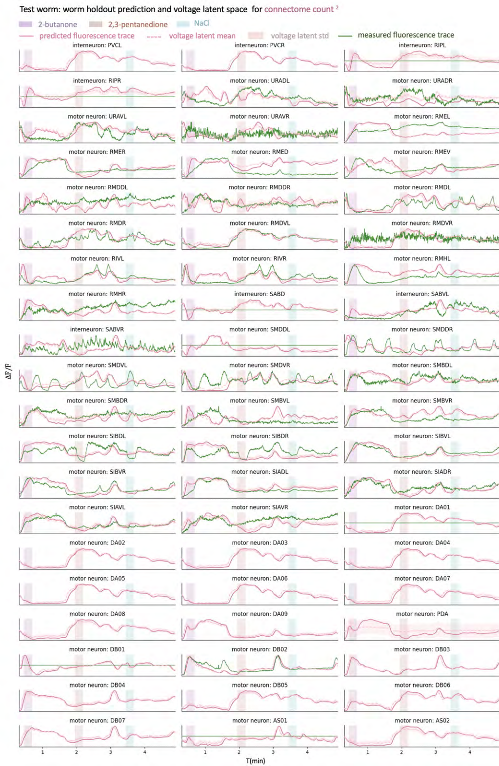
Figure 19: A hold-out (test) worm evaluated on worm holdout using connectome count 2 constraint: CC-LVM predicted traces and the corresponding voltage latent space across all neurons including unmeasured neurons (part 4).
